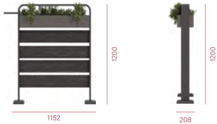
NOMAD DIVIDER WITH PLANTER BOX - 1152 x 1200
