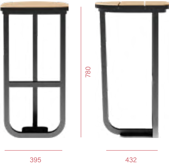
TOBI HIGH STOOL
