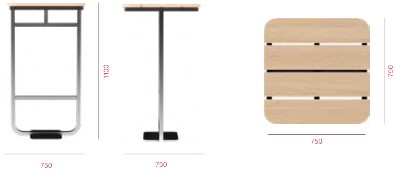
TOBI BARTABLE 750X750
